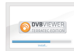
Install Software
