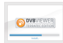
Install Software
